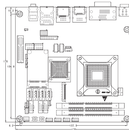
Unit: mm
